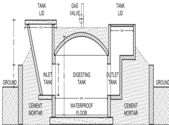
Fig 3: Schematic Diagram of a Janata Biogas Plant
