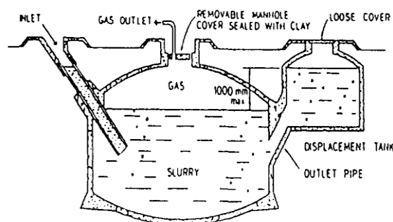
Fig 2: Schematic Diagram of a KVIC Biogas Plant
