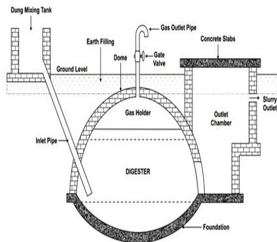
Fig 4: Schematic Diagram of a Deenabandhu Biogas Plant
