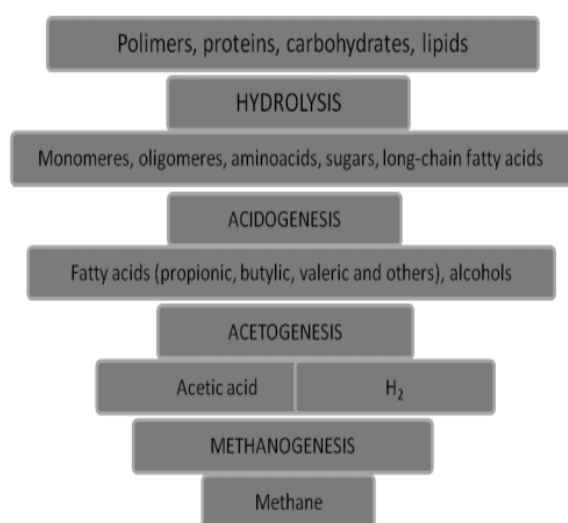
Fig 1: Typical Representation of Anaerobic of Complex Substrates to Biogas
